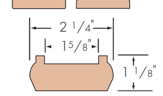
FH6006 Shoe Rail 1 5/8" Plow
