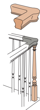
FH7021 Quarterturn Cap *available in 135°
