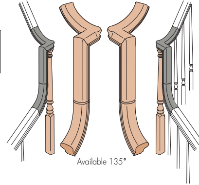
Newel F7060 Left Hand 2-Rise with Cap
