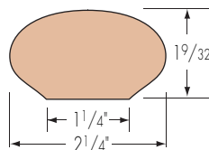
F6042 Wall Rail
