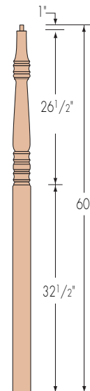
F4215 Landing Newel 3 1/2"
