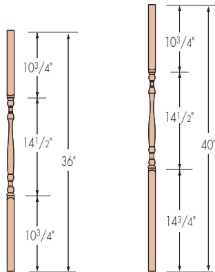
FH5801-36 1-1/4" Sq. FH5801-40 1-1/4" Sq. Use with non plow handrail
