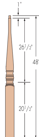
F4220 Starting Newel 3 1/2"
